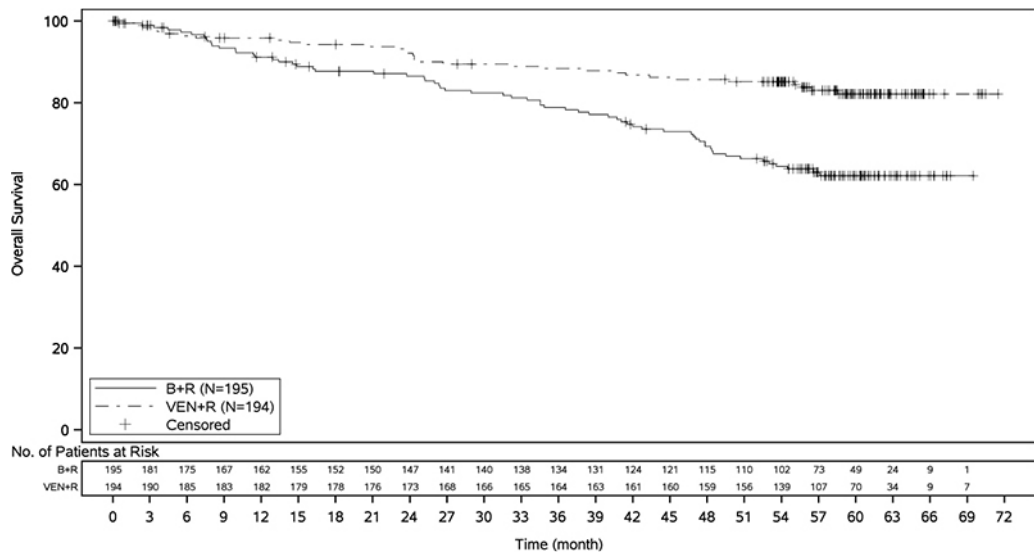
Figure 3. Kaplan-Meier Curve of Overall Survival in MURANO
