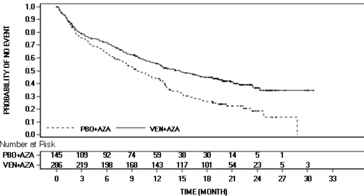
Figure 4. Kaplan-Meier Curve for Overall Survival in VIALE-A
